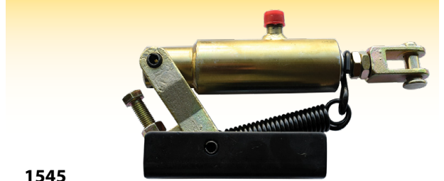
1545 Trailer Brake Ram with Bracket
