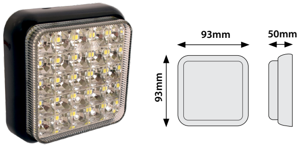
55210 LED Reverse Lamp 10-30V 40cm Cable
