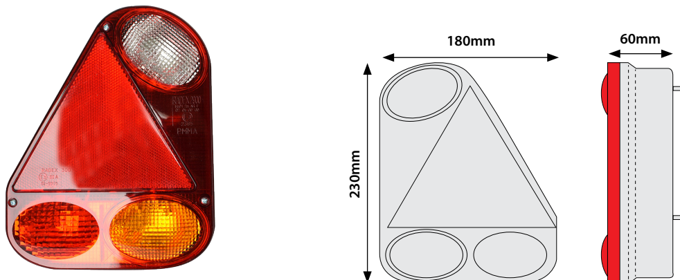
55214 Combination Lamp Rectangular 12V Bulbs Included
