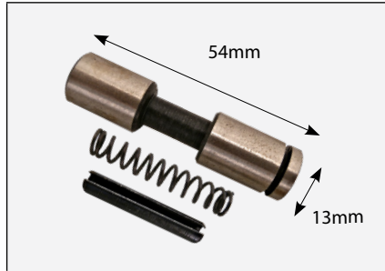
1456 PTO Release Button 13 x 54mm Flat Head
