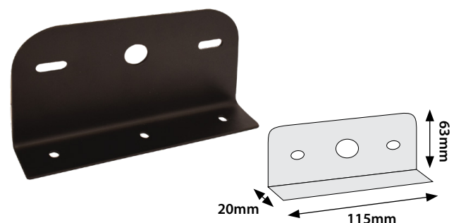
55219 Mounting Bracket For 55218 12mm Hole Diameter
