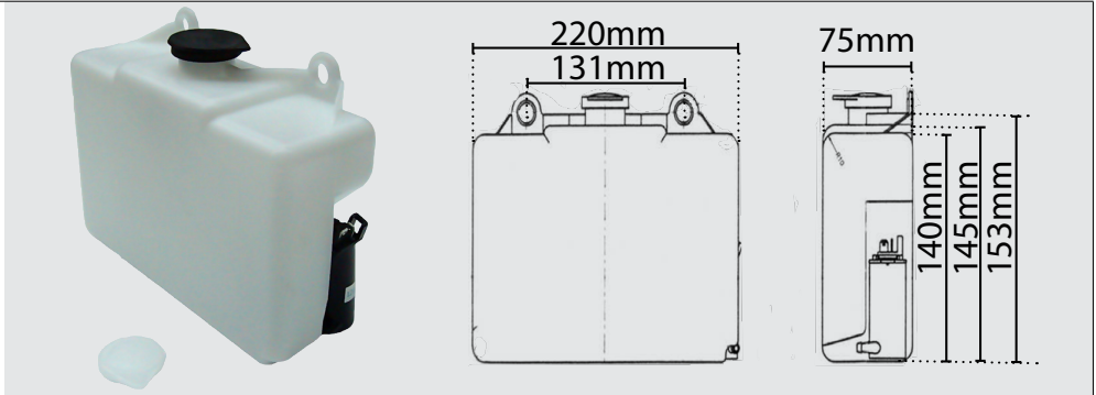
51080 Window Washer 2.2 Ltr 12V 220 long x 153 high x 75mm wide
