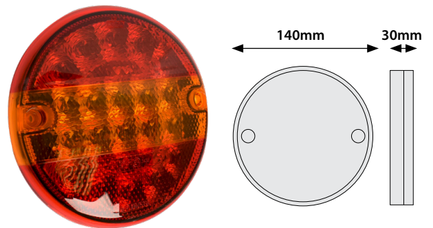
55206 LED Combination Lamp Round 9/30V Spade Connection
