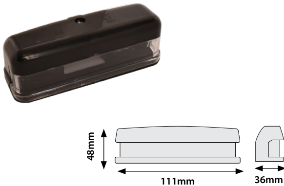
55217 Number Plate Lamp 12V With Studs & Bulbs Included
