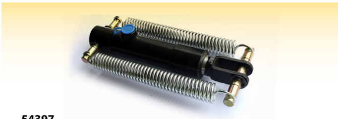
54397 Trailer Brake Ram 30mm Double Spring Return 75mm Stroke
