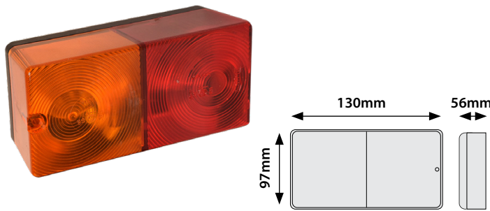
55214 Combination Lamp Rectangular 12V Bulbs Included
