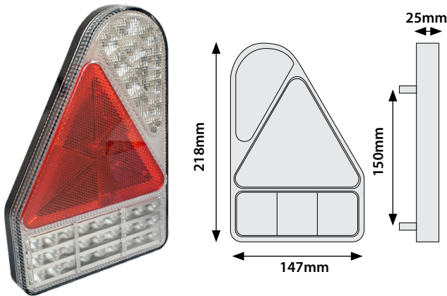
LED Combination Lamp Triangle Slimline Chrome 10/30V 45cm Cable
