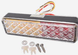
55687 LED Rear Lamp Stop Tail Indicator 12/24V 135mm x 38mm x 24mm
