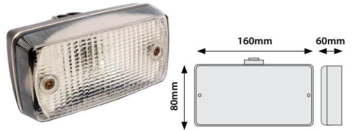
55216 Reverse Lamp 12V with Mounting Bracket Bulbs Included
