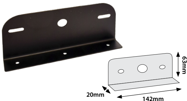
55220 Mounting Bracket 12mm Hole Diameter
