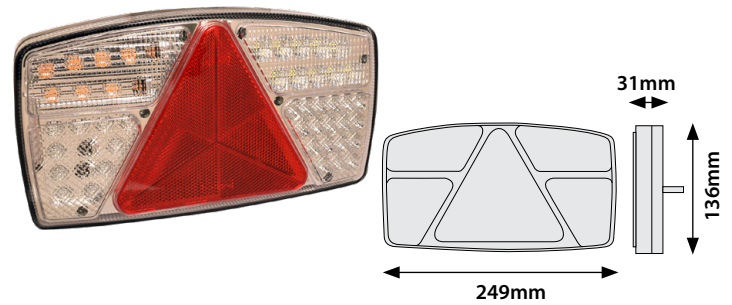
LED Combination Lamps 10/30V 54cm Cable
