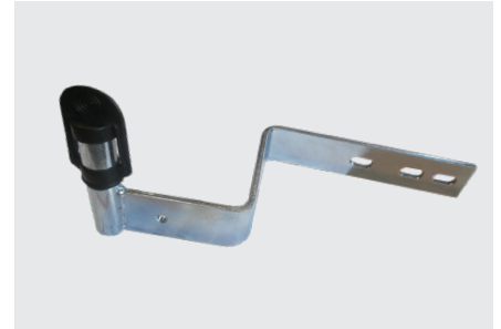
43190 Left Hand Beacon Bracket Assembly Ford 5640 6640 7740 7840 8240 8340
