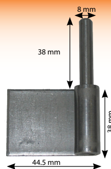
3184 Hinge Male Lift Off LH
