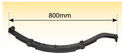
51444 Multi Leaf Trailer Spring 5 Leaf Spring
