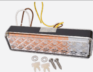
55688 Front Marker Lamp LED 12/24V 135mm x 38mm x 24mm
