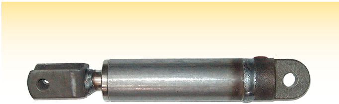
4611 Trailer Brake Ram Cylinder 25mm 285mm centres 70mm Stroke with Internal Return Spring
