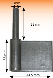
3185 Hinge Male Lift Off RH
