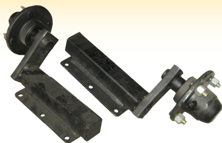
51135 Trailer 350kg Suspension Unit Per Pair 4" PCD Hubs 4 Stud Grease Nipples
