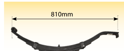
51650 Multi Leaf Trailer Spring 7 Leaf Spring
