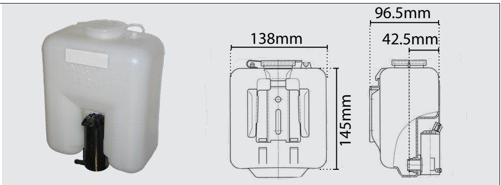
51607 Window Washer 12V 138 long x 125 high x 97mm wide
