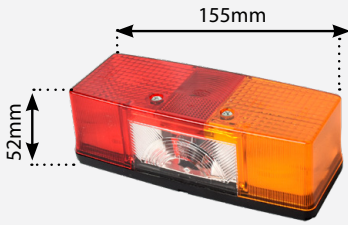
3646 Rear Lamp Left Hand with Number Plate Lamp Lens is 3648
