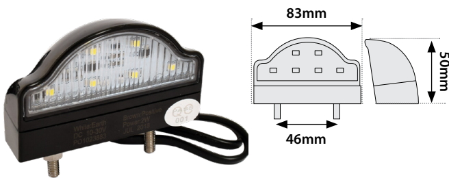
55211 LED Number Plate Lamp 10-30V 32cm Cable With Mounting Bolts
