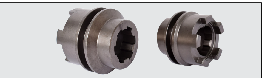
67157 PTO Coupling Sleeve Landini Powerfarm 60 - Powerfarm 105 Globalfarm 90-105 OE Ref: 3691665M1
