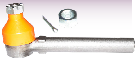
3195 Track Rod End 3050 3060 3065 Length: 200mm - Thread: M18 x 1.5mm
