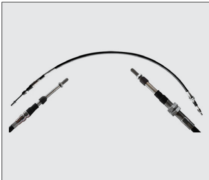
52808 Shuttle Cable Powerfarm Landini Vision OE Ref: 4208518M91
