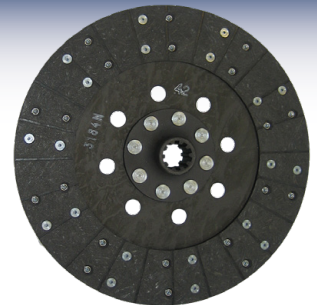
1616 Main Disc Leyland David Brown 12' PTO Drive 12" x 1 1/8" (10 Splines)
