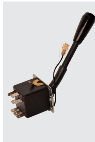
54973 Indicator & Lighting Switch Deutz 07 07C OE Ref: 04319505
